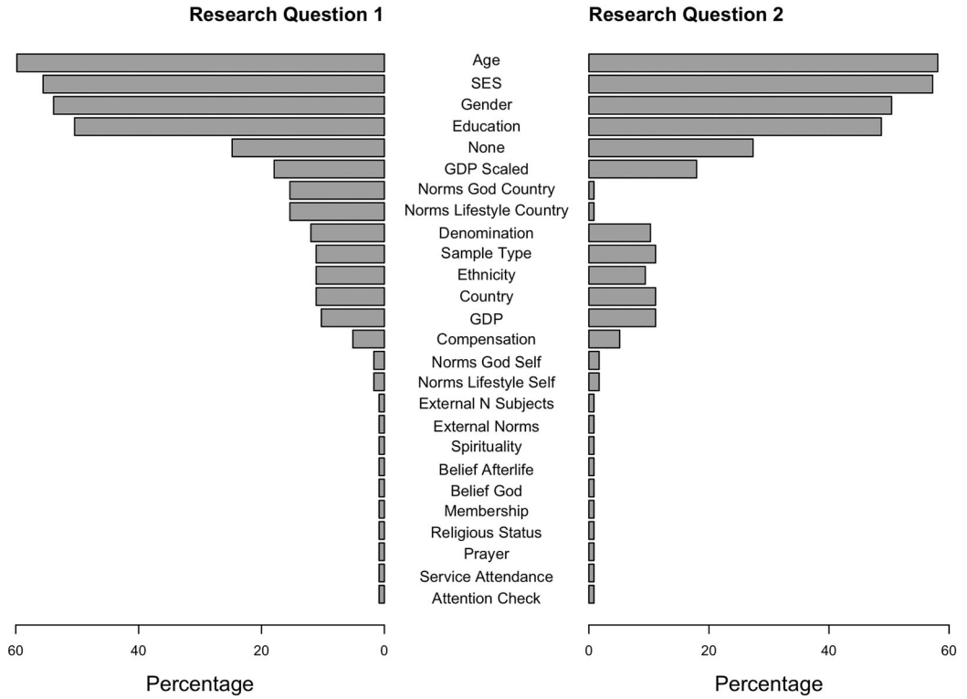
Figure 9. Items included as covariates for research question 1 (on the left) and research question 2 (on the right). Variables indicated as “external” refer to covariates that are based on data not provided by the MARP team.
